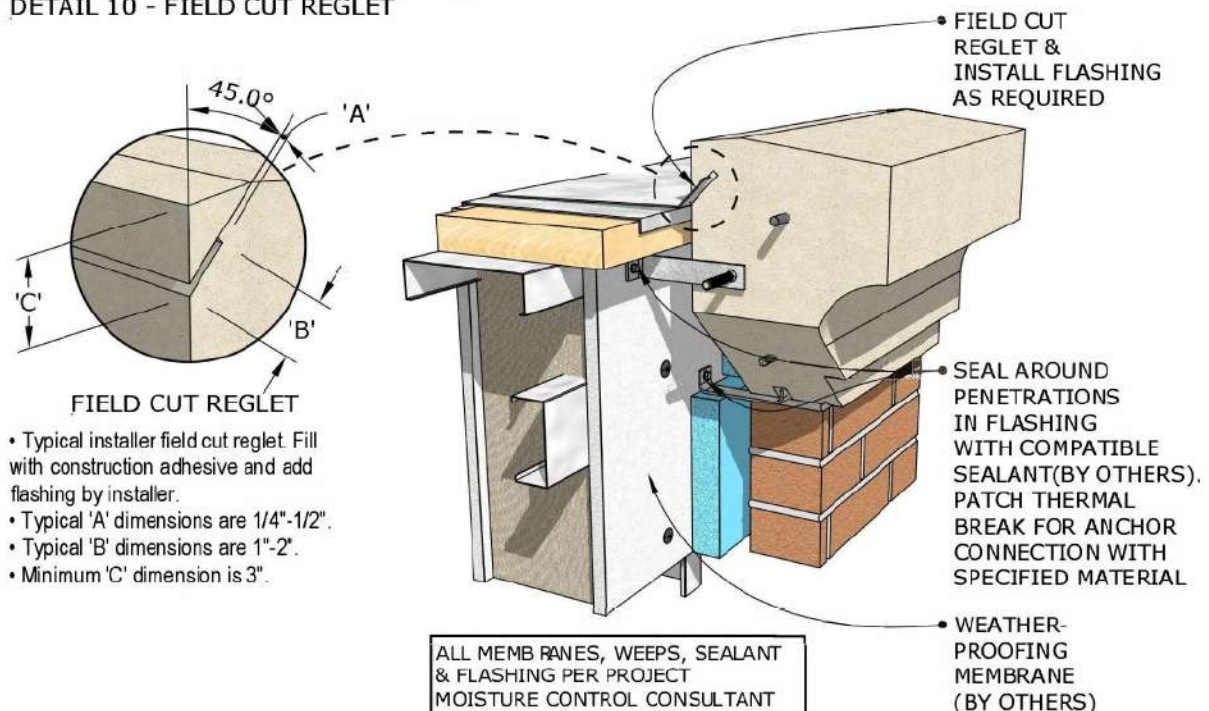
DETAIL 10 - FIELD CUT REGLET
