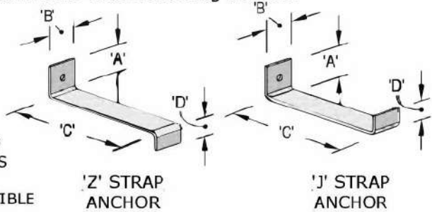
DETAIL 1 - 'Z' & 'J' STRAP ANCHOR @ HEADER
